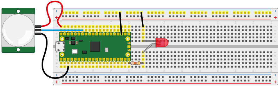
▲ Figure 7-2: Adding an LED to the burglar alarm
